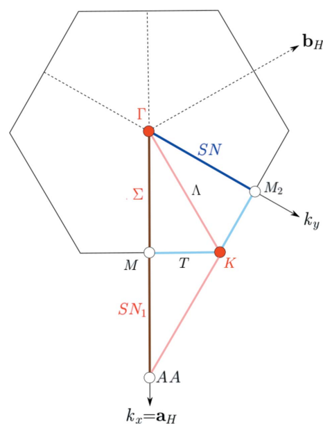
Figure 8 Brillouin zone and representation domain of LW, and asymmetric unit of the layer group p\bar{6}2m (No. 78). The reciprocal plane group is (p31m)^* (No. 15). The representation domain of LW is different from the asymmetric unit.
