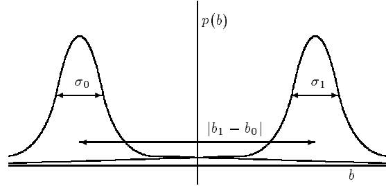
Probability densities p of B according to input |\psi_0\rangle and |\psi_1\rangle
