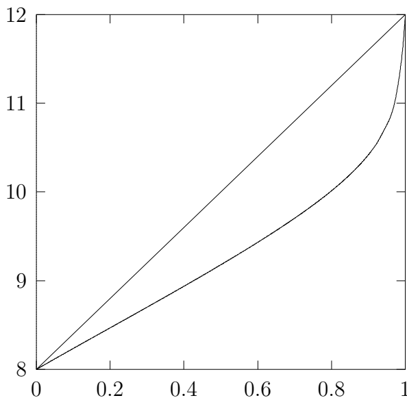
Figure 2: The fourth moment of X + Y and \gamma(X) + Y for q \in (0, 1) .
