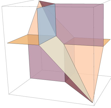
FIGURE 1. The cell decomposition for a matroid flock of U_{2,4} ; the two zero-dimensional cells are 0 and -ge_2 - ge_3 .
