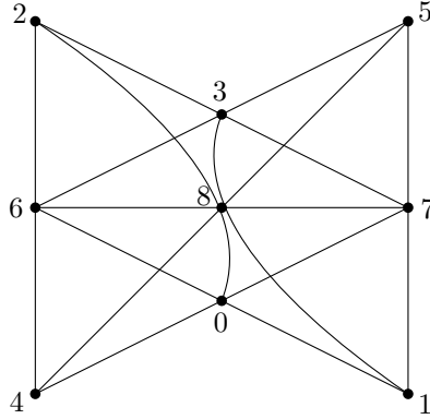
FIGURE 1. The quaternary butterfly, a rank 3 matroid on 9 elements. A triple is a non-basis if and only if it is connected by a line.
