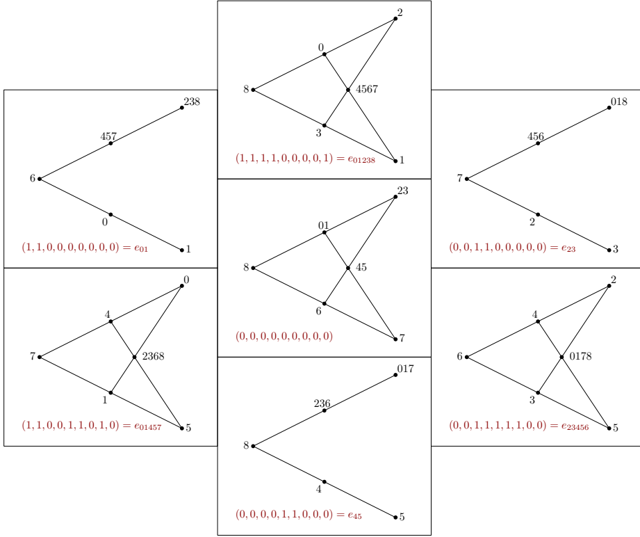
FIGURE 2. The central points of \mathcal{M}^{\nu_Q} .
