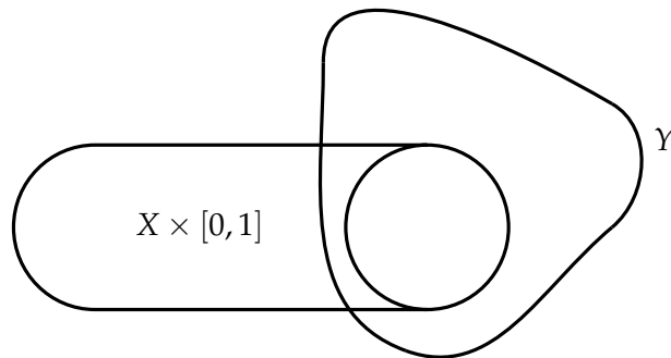
Figure 15.1: The mapping cylinder of f: X \rightarrow Y
