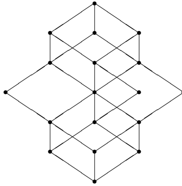
Figure 6: The free distributive lattice on three elements.
